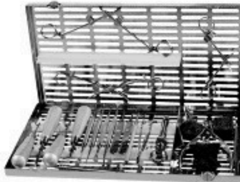
786-1587 Oral Surgery Kit (C) Exterior Dimensions 14.5" x 8" x 1.25" (368mm x 203mm x 32mm)
